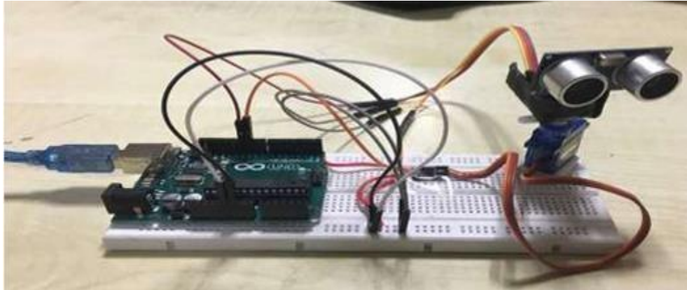
Figure 8. Breadboard of the hardware system implementation
