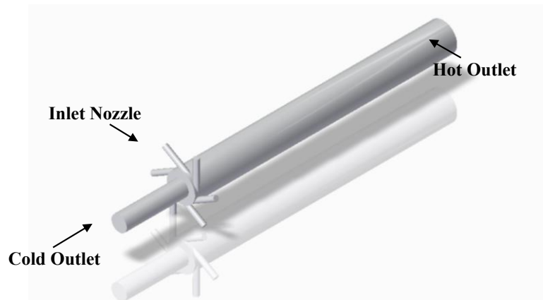
Figure 2. 3-D model of a vortex tube with inlet and exit conditions
