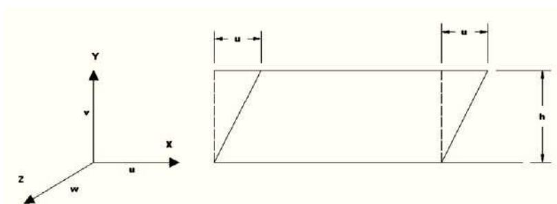
Figure 2. Fluid film depicting the Shear
