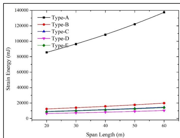
Figure 6. Effect of maximum strain energy due to IRC Class AA Loading condition in different types of bridge deck with variation of bridge span length
