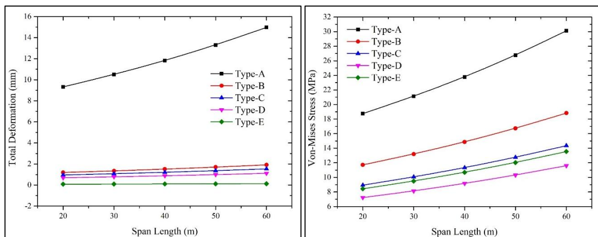
Figure 4. Effect of maximum total deformation and von-mises stresses due to IRC Class AA Loading condition in different types of bridge deck with variation of bridge span length
